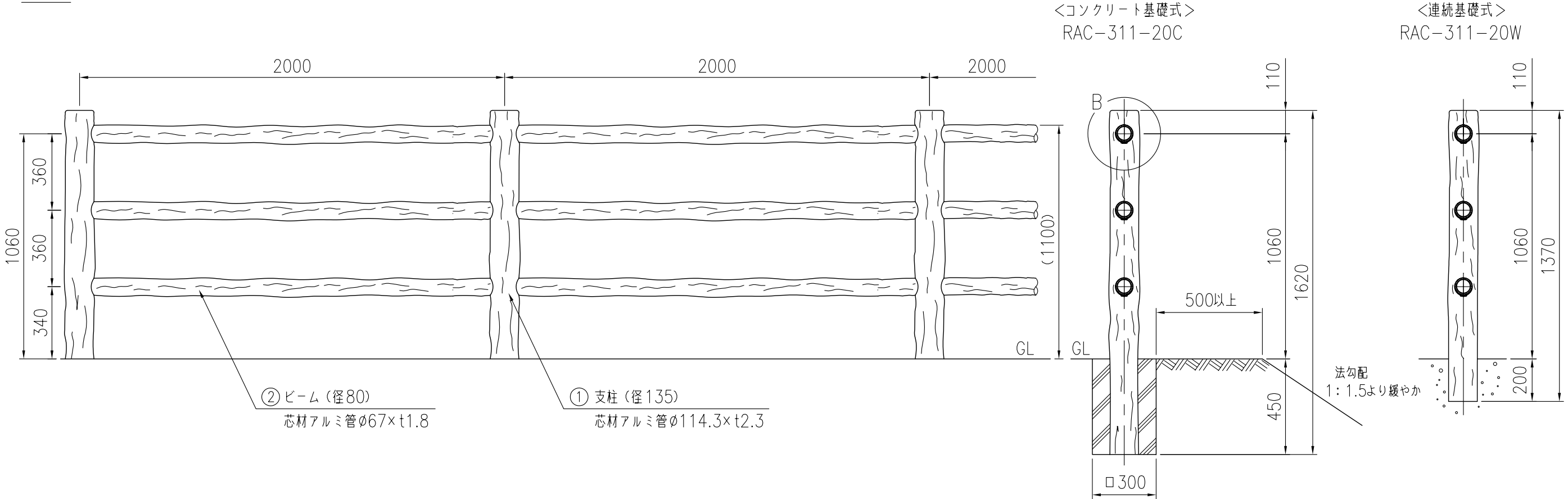
取付部詳細 (1/4)
