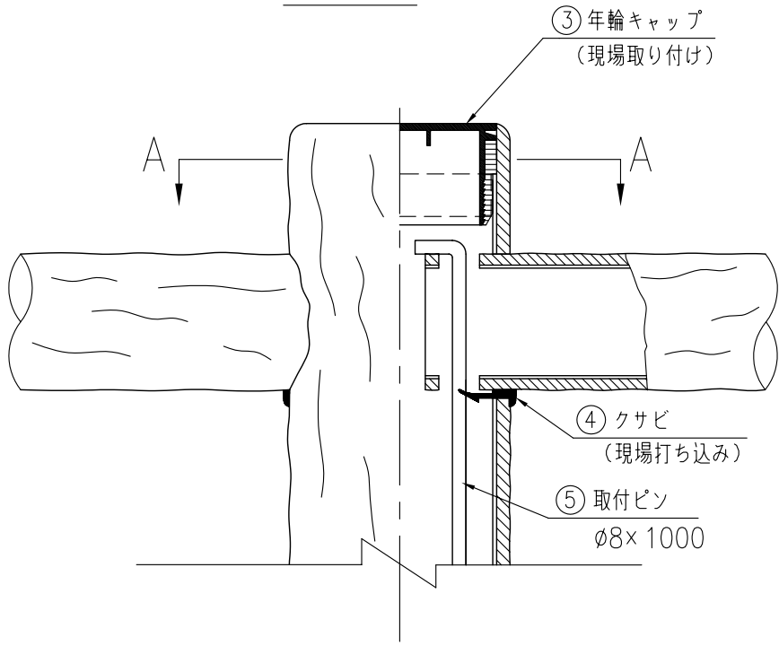
取付部詳細 (1/4)
