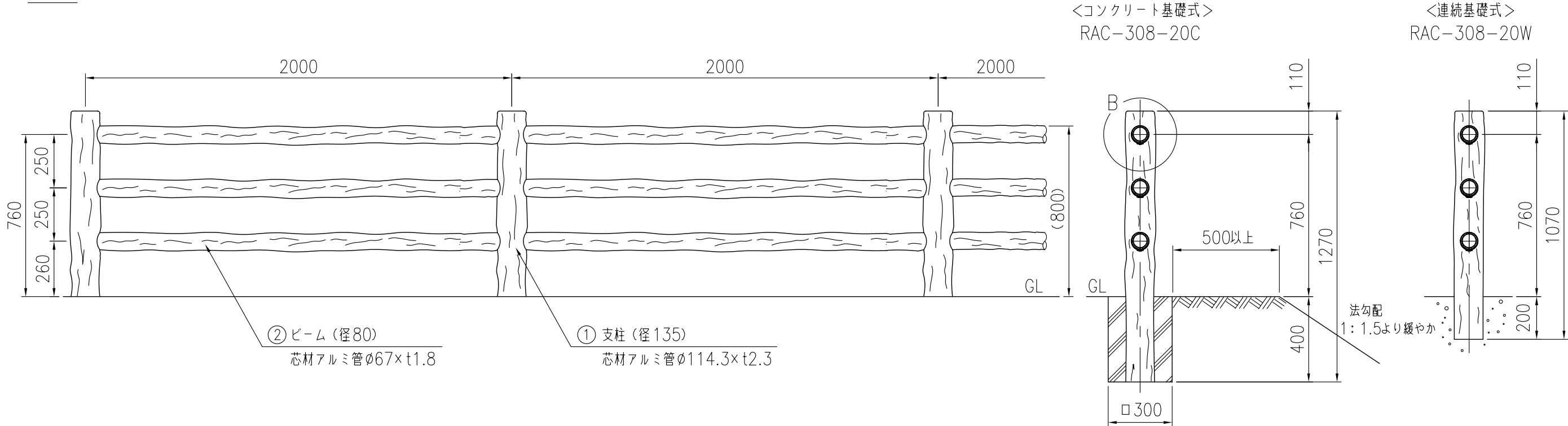
取付部詳細 (1/4)
