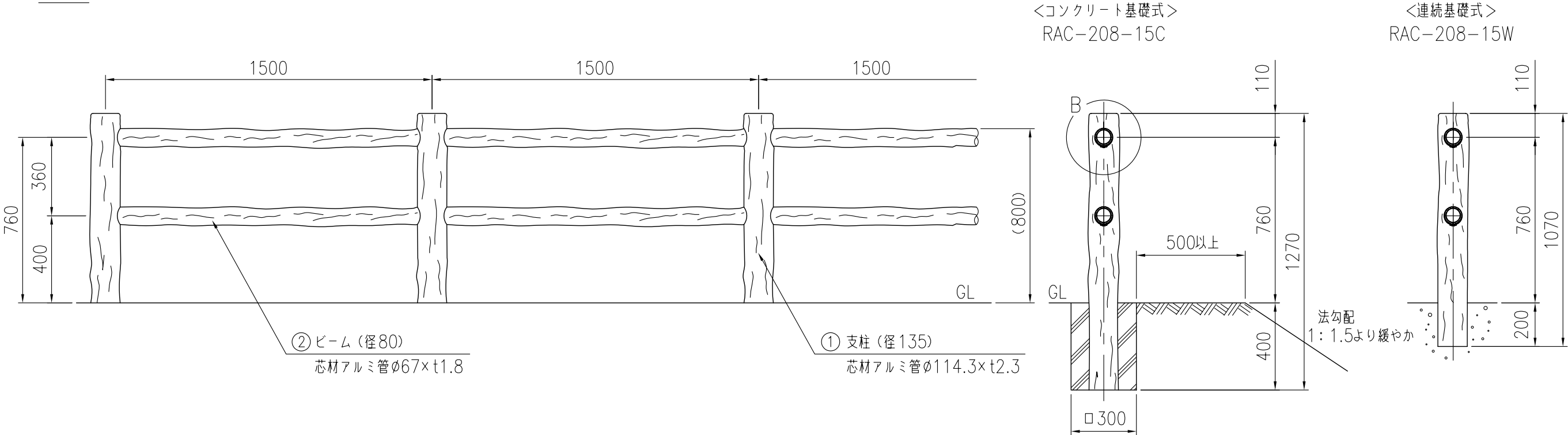
取付部詳細 (1/4)
