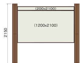
SOW-NAH1221-1S(W)
