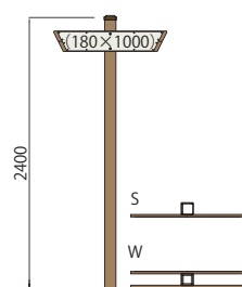
TW-KH0210-1S TW-KH0210-1W
