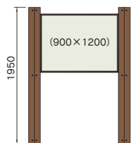
SOW-NA0912-1S(W)
