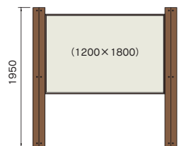
SOW-NA1218-1S(W)
