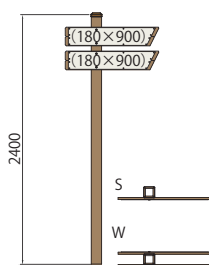
TW-YH0209-2S TW-YH0209-2W
