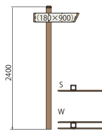
TW-YH0209-1S TW-YH0209-1W
