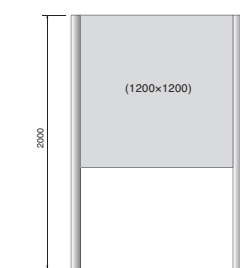
SUS-M1212-S(W)
