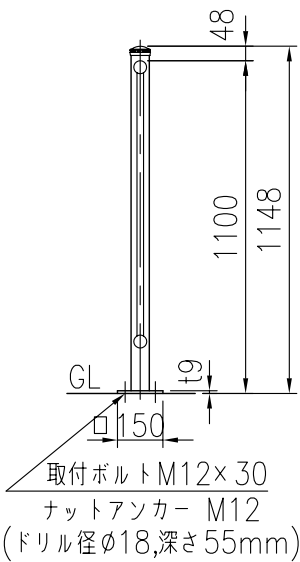
FT-40AP111PL20
