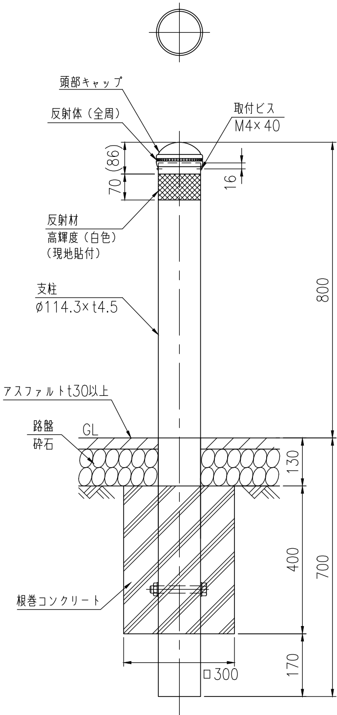
KDK-F114SE(1/10)
