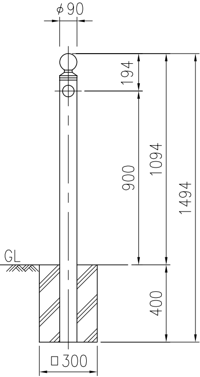
CR1-1S89
