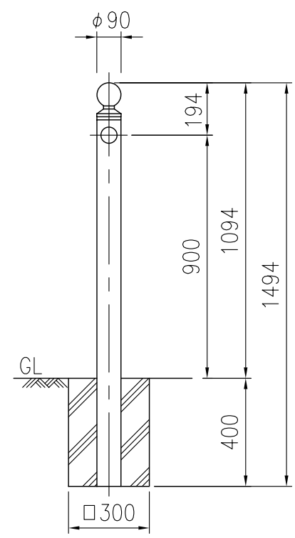
CR1-1A89
