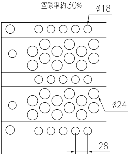
A部詳細 (1/5)
